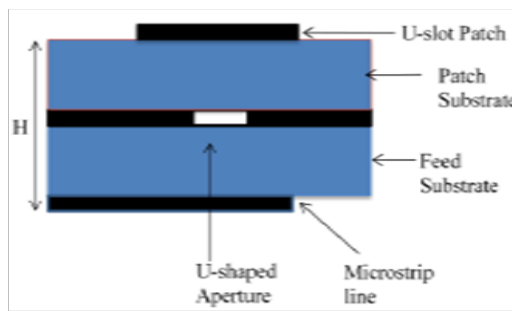
Fig. 1 Geometry of aperture coupled antenna
